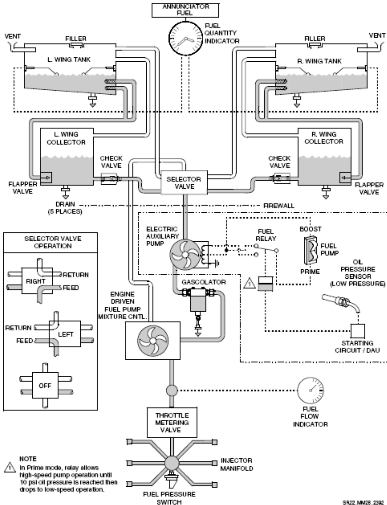
Figure 28-002 Fuel System Schematic - Serials 2438 & subs (Sheet 2 of 2)
